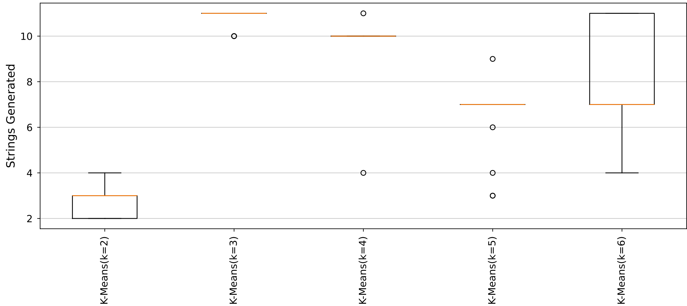
YARA Rules Strings Generated Distribution (Cluster33_Size6 dataset)
